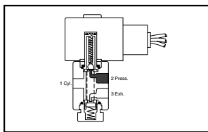
Figure 5A: Three-Way Normally Closed Valve, De-Energized
